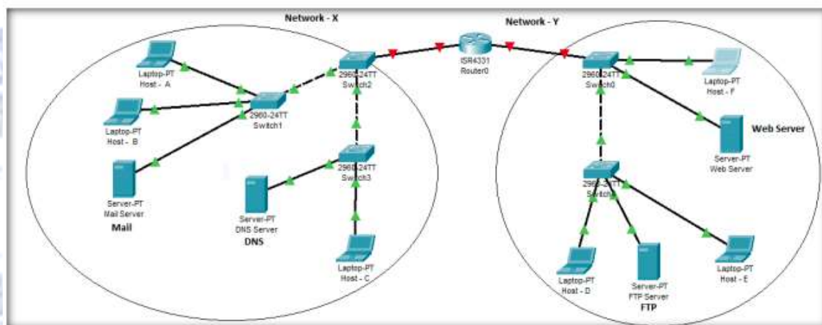
Figure # 01: Network Topology
